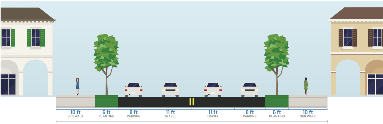
Representative section at a typical right-of-way; widths are typical values within the ranges in the Design Standards below. Cross-section illustration adapted from Streetmix (streetmix.net), © the Streetmix project, licensed CC BY-SA 4.0.
